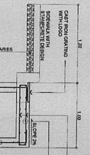
SECTION OF RCBC-1 SCALE 1:20M
